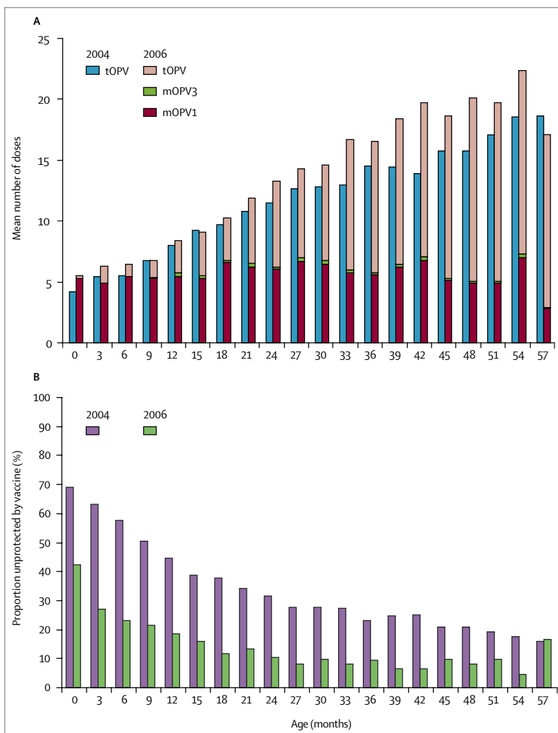
Figure 1: The effect of monovalent vaccine on population immunity among children in Uttar Pradesh Calculations assume that all doses were received through supplementary immunisation campaigns. (A) The mean number of doses of each type of oral poliovirus vaccine received by children in Uttar Pradesh by 3-month age-groups, comparing the last quarter of 2004 with 2006. (B) The proportion of children in Uttar Pradesh who remained unprotected by oral vaccine against type 1 paralytic poliovirus in the last quarter of 2004 and 2006, based on the estimated coverage and efficacy of monovalent and trivalent vaccines. mOPV1=monovalent oral type 1 poliovirus vaccine. mOPV3=monovalent oral type 3 poliovirus vaccine. tOPV=trivalent oral poliovirus vaccine.
